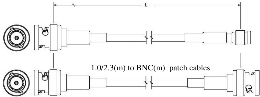
BNC(m) to BNC(m) patch cables
